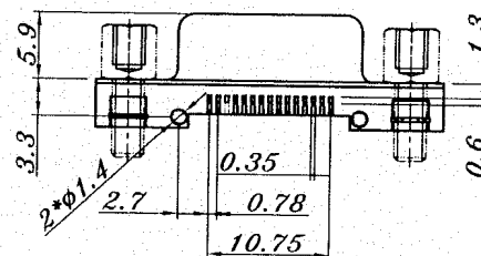
427B Socket
