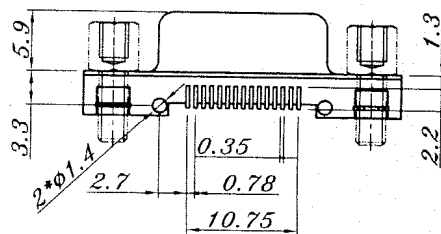
427A Socket
