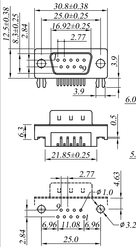
P.C.B LAYOUT TO SUGGEST
