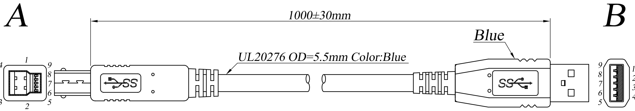
USB3.0 B-TYPE Plug
