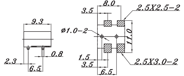
P.C.B LAYOUT BOTTOM VIEW
