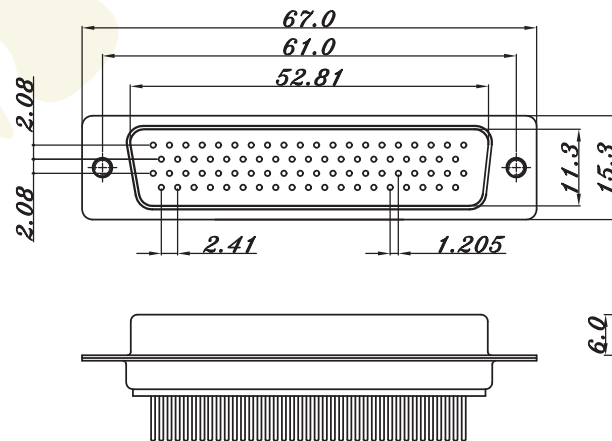
50 POSITION MALE
