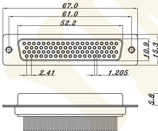
50 POSITION FEMALE
