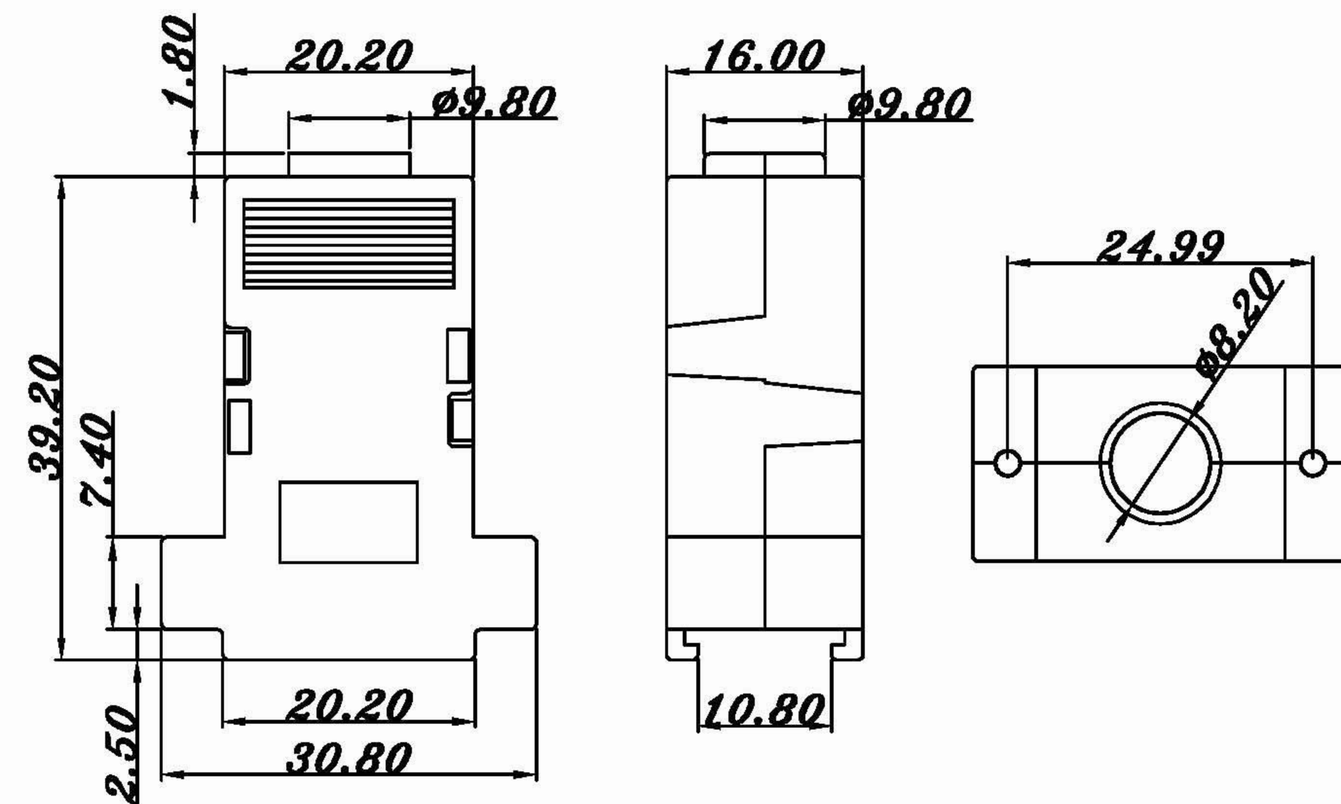
Snap-In Type 9 Pin
