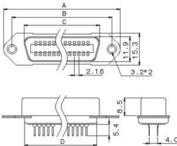
FEMALE W/O LATCH
