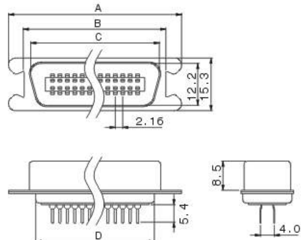
MALE-MOLDED TYPE
