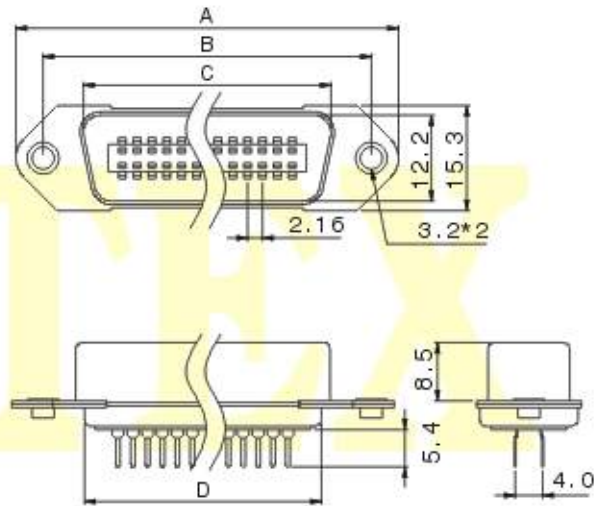
MALE W/O LATCH
